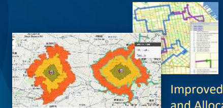
Contour Polygons
